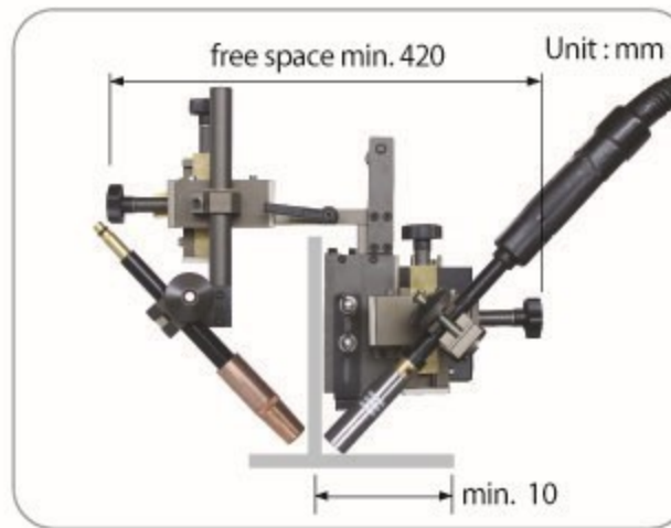
FILLET WELDING
