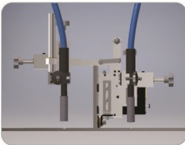
BUTT WELDING
