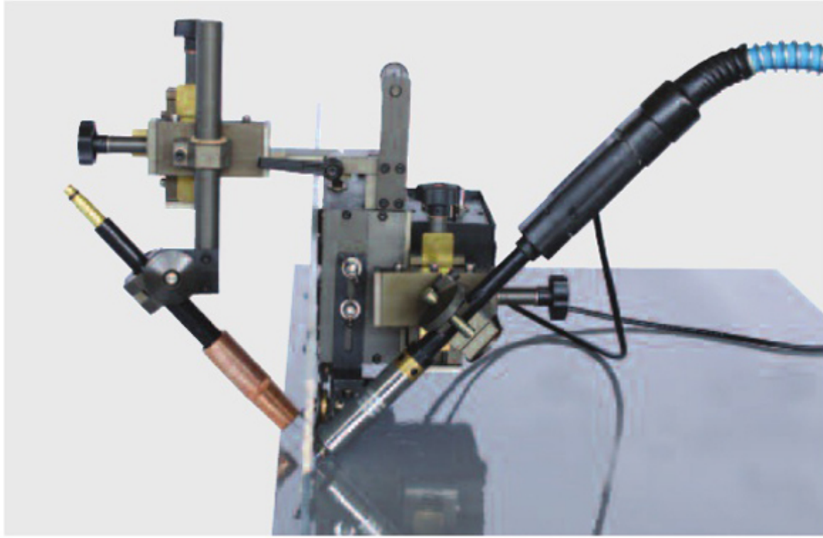
BUTT WELDING
