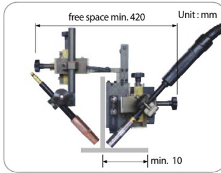
FILLET WELDING
