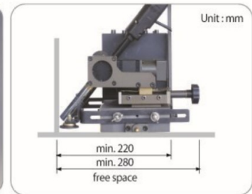
VERT-UP FILLET WELDING
